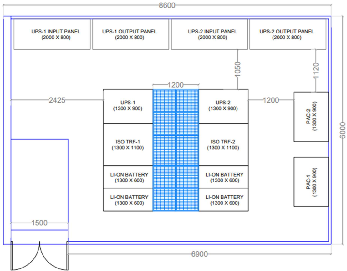
TENTATIVE LAYOUT OF UPS ROOM AT BASEMENT
