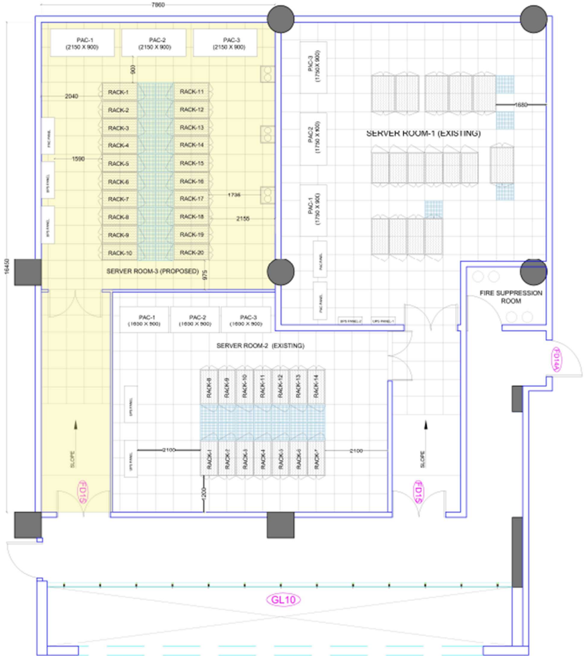
TENTATIVE LAYOUT OF SERVER ROOM AT SECOND FLOOR
